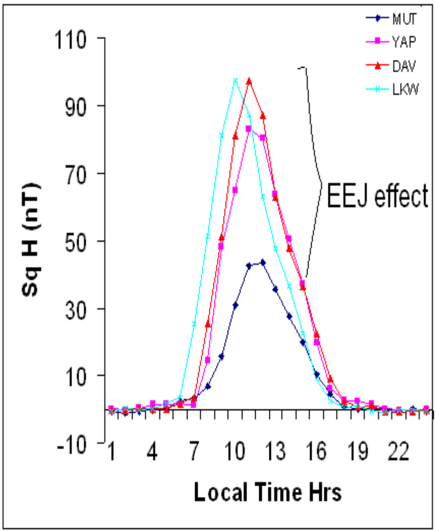
Sq variation in Hon 2nd April 08 (Ap=1)
