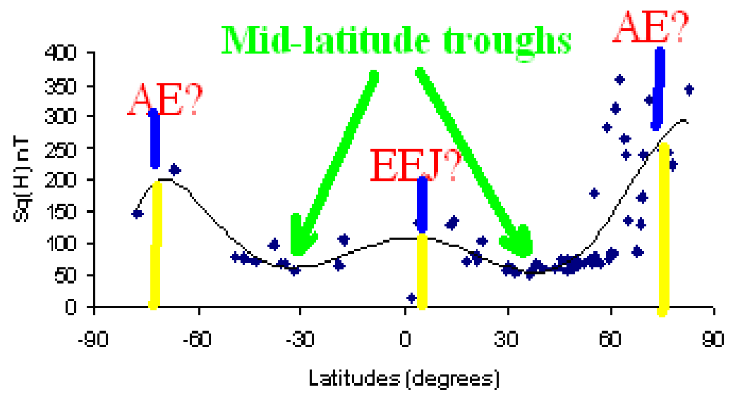
Latitudinal variation of Annual Sq 1996
