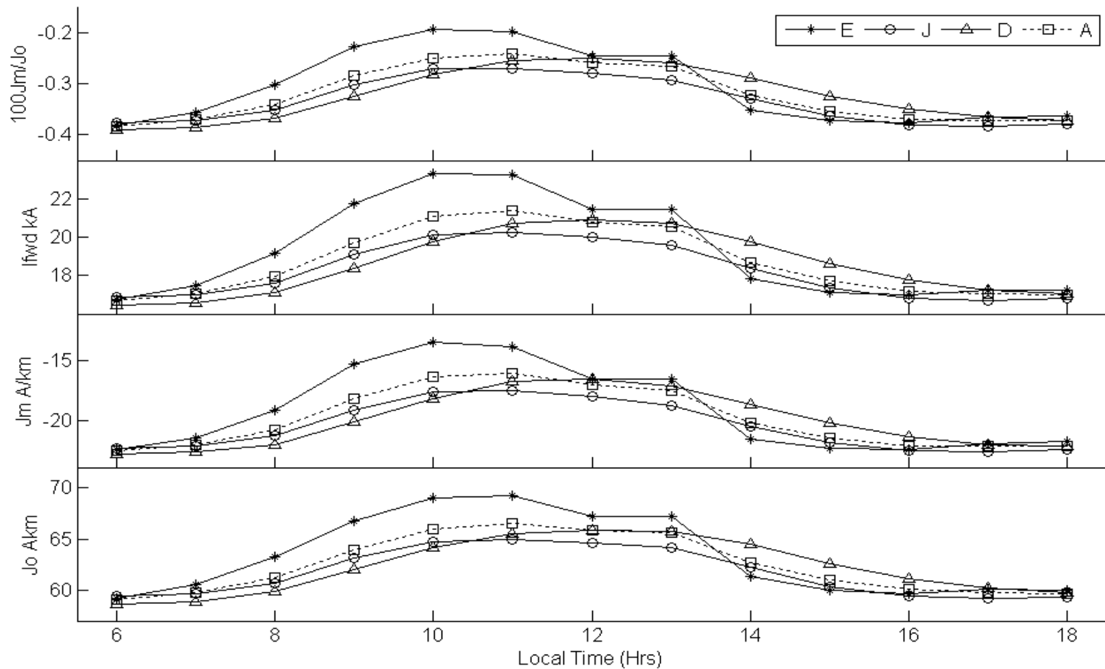
Diurnal variations of the landmark measures of the of EEJ current over India.
