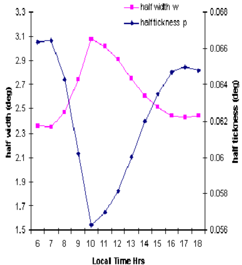
Half width and half thickness of EEJ
